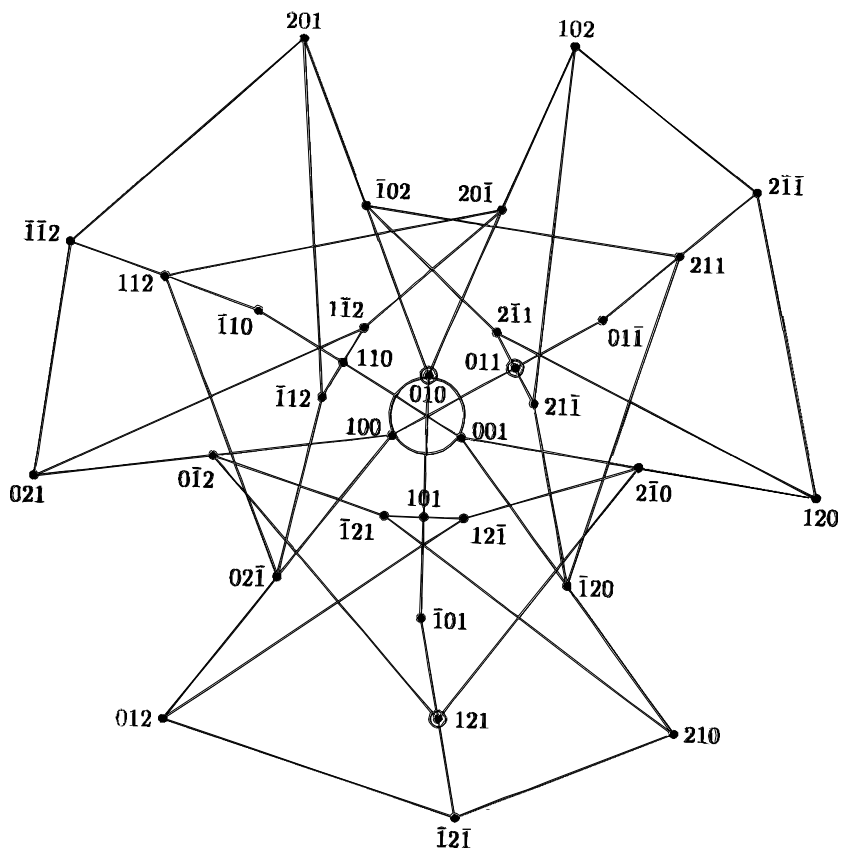
Fig. 3 'Almost' Greechie diagram of a suborthoposet of L(\mathbb{R}^3) without any two-valued state [e.g., 121 = \text{Sp}(1, \sqrt{2}, -1) ].
