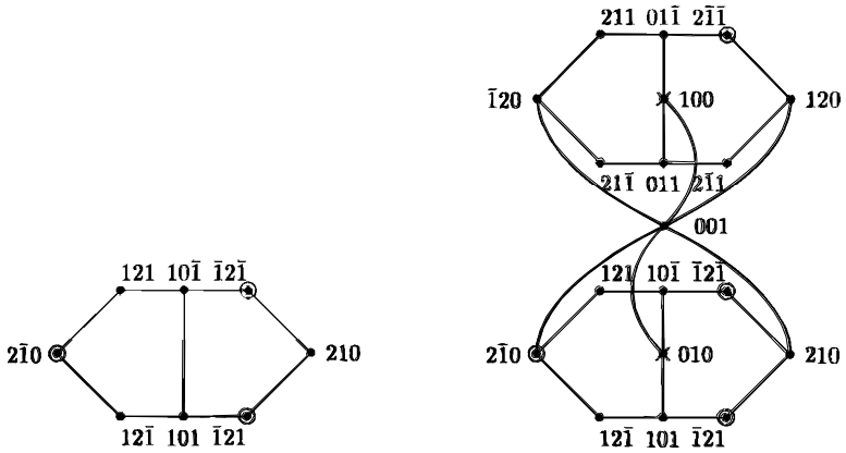
Fig. 1 ‘Almost’ Greechie diagrams of suborthoposets of L(\mathbb{R}^3) without a full and without a separating set of two-valued states [e.g., 121 = \text{Sp}(1, \sqrt{2}, -1) ].
