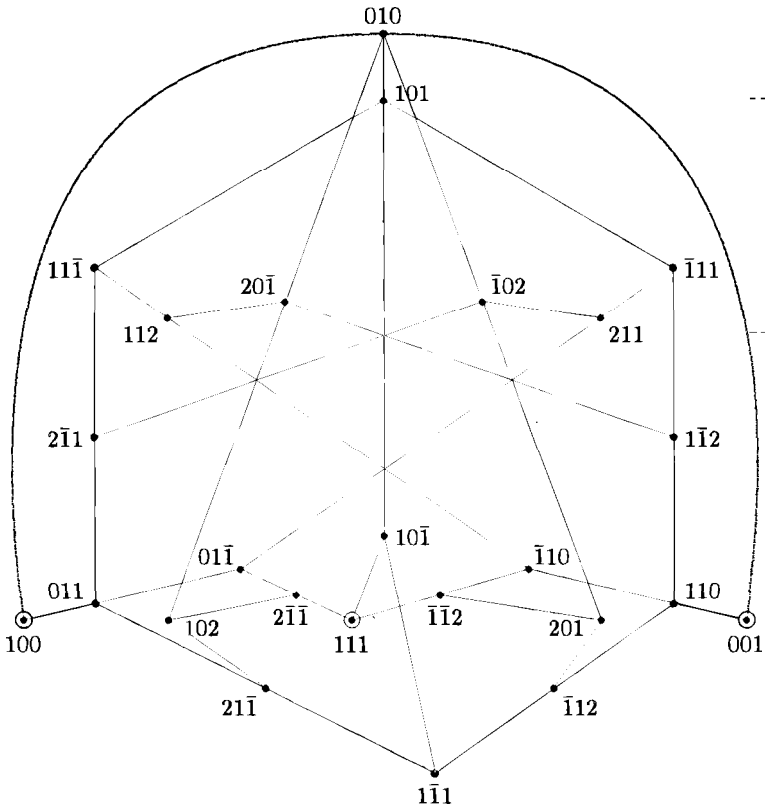
Fig. 2 ‘Almost’ Greechie diagram of a suborthoposet of L(\mathbb{R}^3) without a unital set of two-valued states [e.g., 121 = \text{Sp}(1, 2, -1) ].
